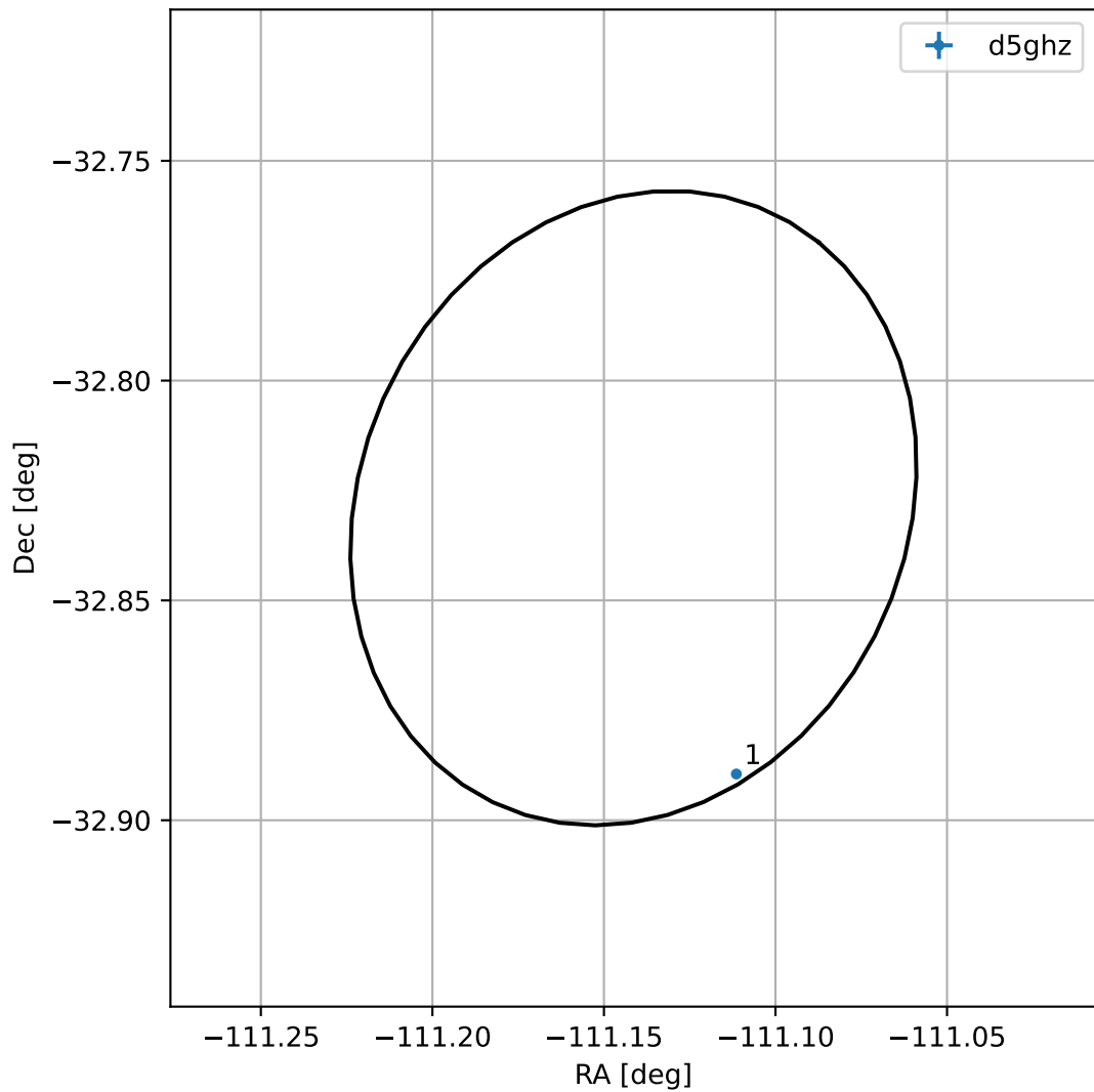
4FGL J1635.4-3249
