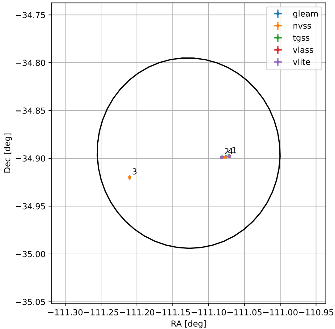
4FGL J1635.4-3453
