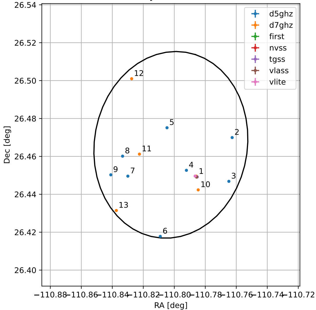
4FGL J1636.7+2627
