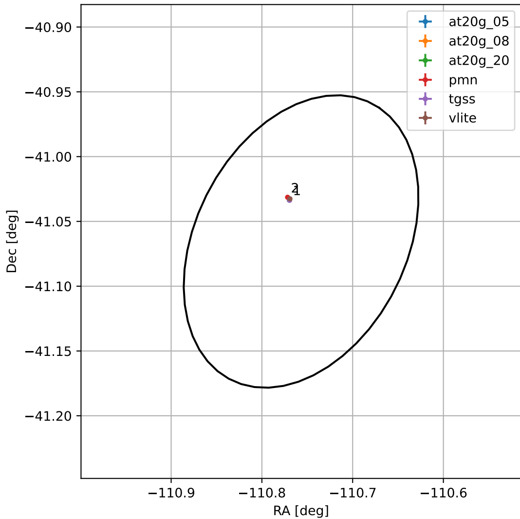
4FGL J1636.9-4103
