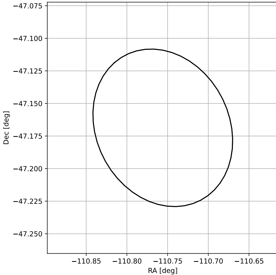
4FGL J1636.9-4710
