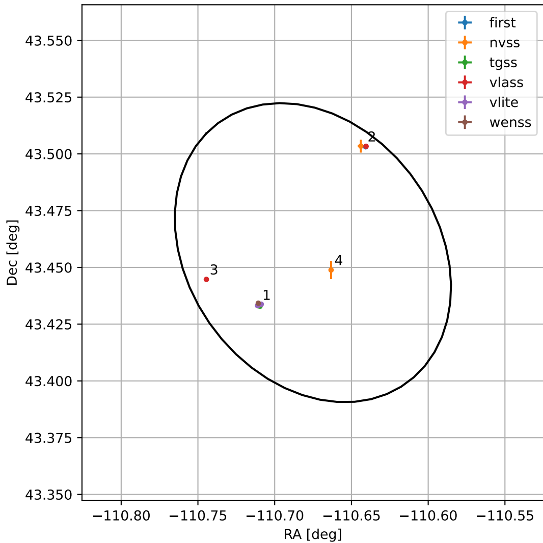
4FGL J1637.2+4327
