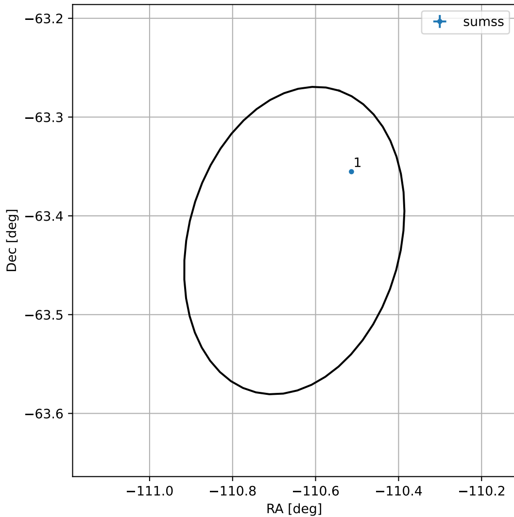
4FGL J1637.3-6325
