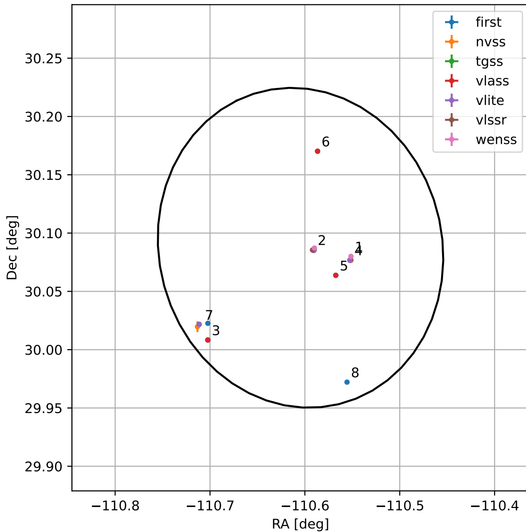
4FGL J1637.5+3005
