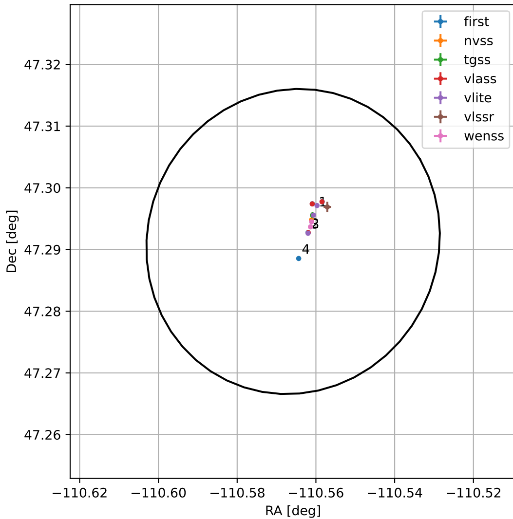
4FGL J1637.7+4717
