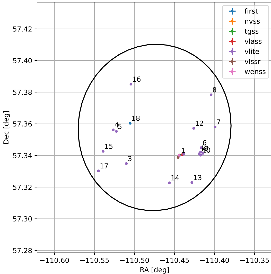
4FGL J1638.1+5721
