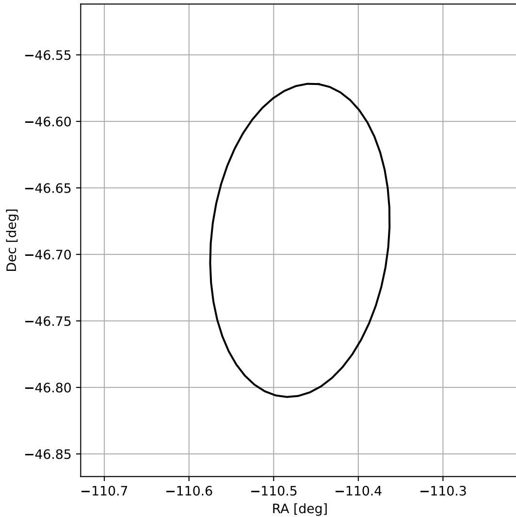
4FGL J1638.1-4641
