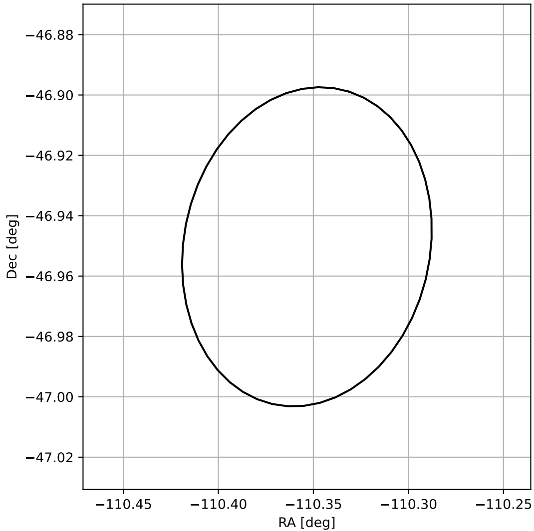
4FGL J1638.5-4657
