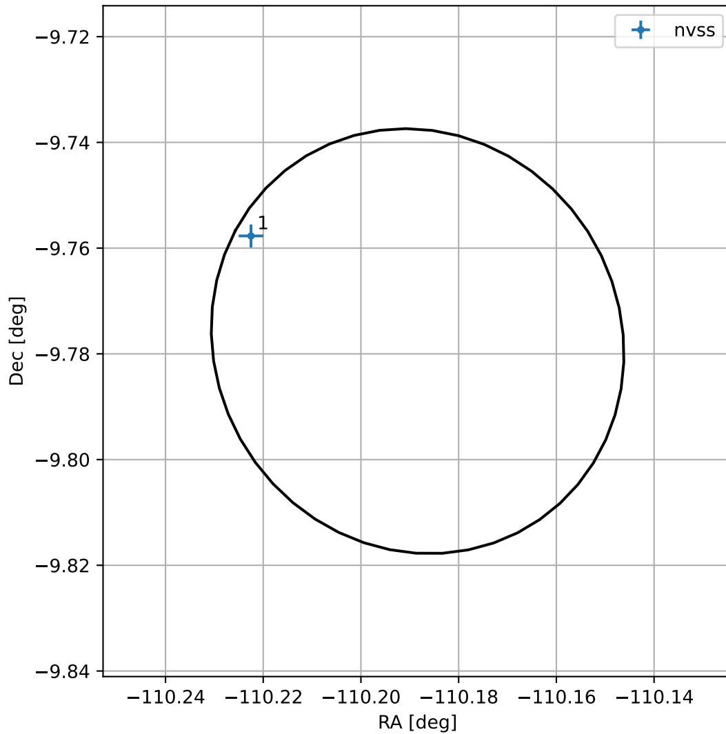
4FGL J1639.2-0946
