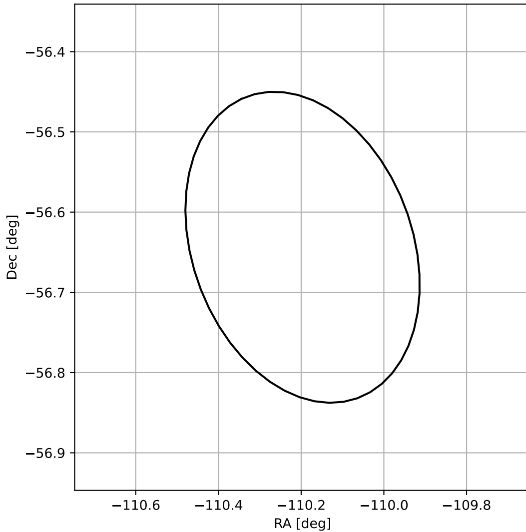
4FGL J1639.2-5638
