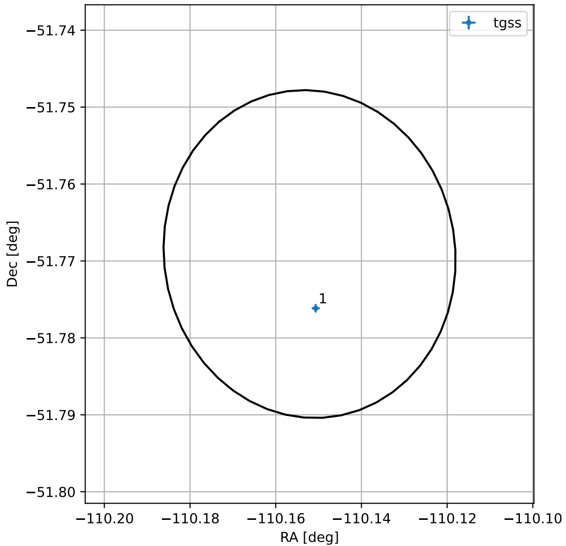
4FGL J1639.3-5146
