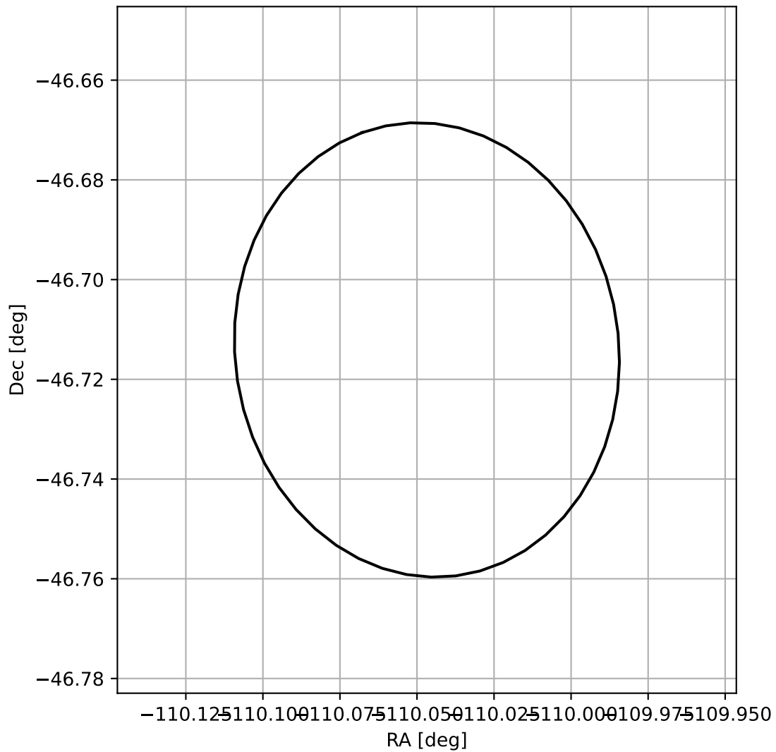
4FGL J1639.8-4642
