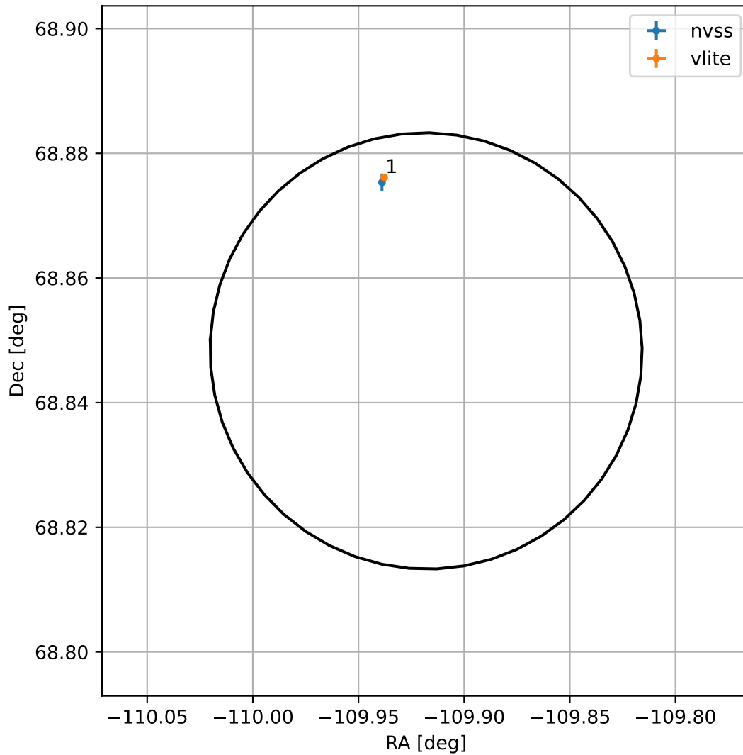
4FGL J1640.3+6850
