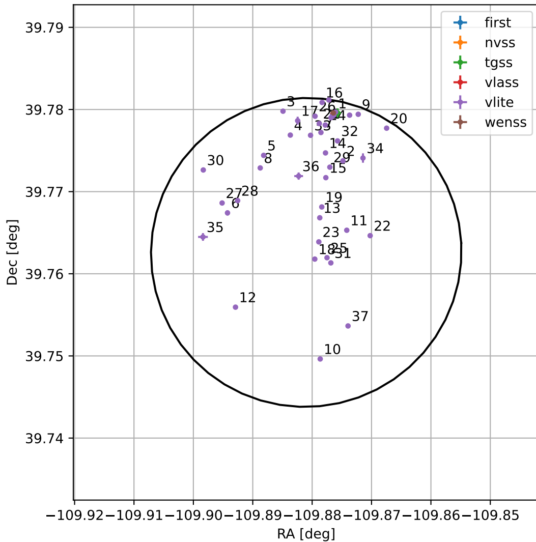
4FGL J1640.4+3945
