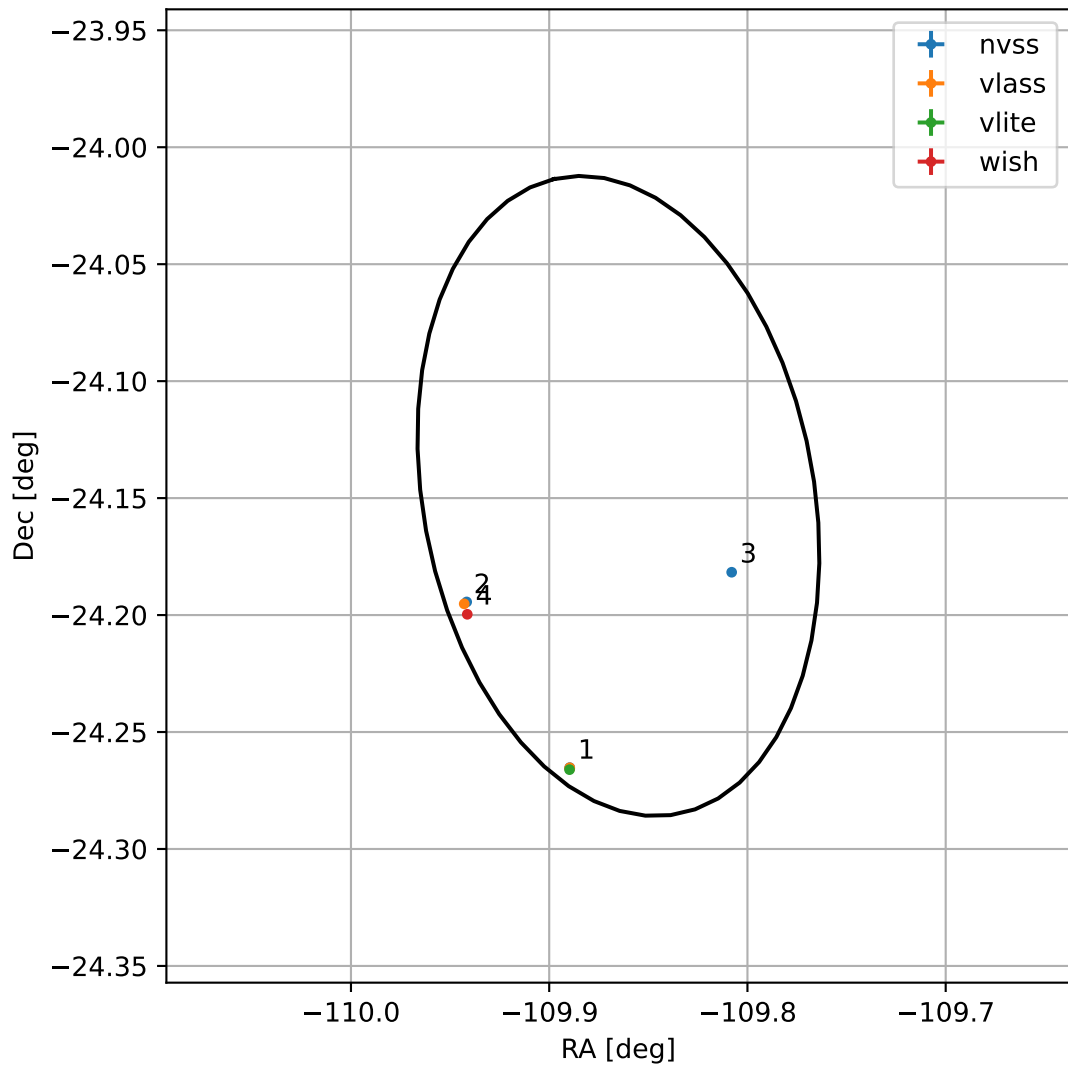
4FGL J1640.5-2408
