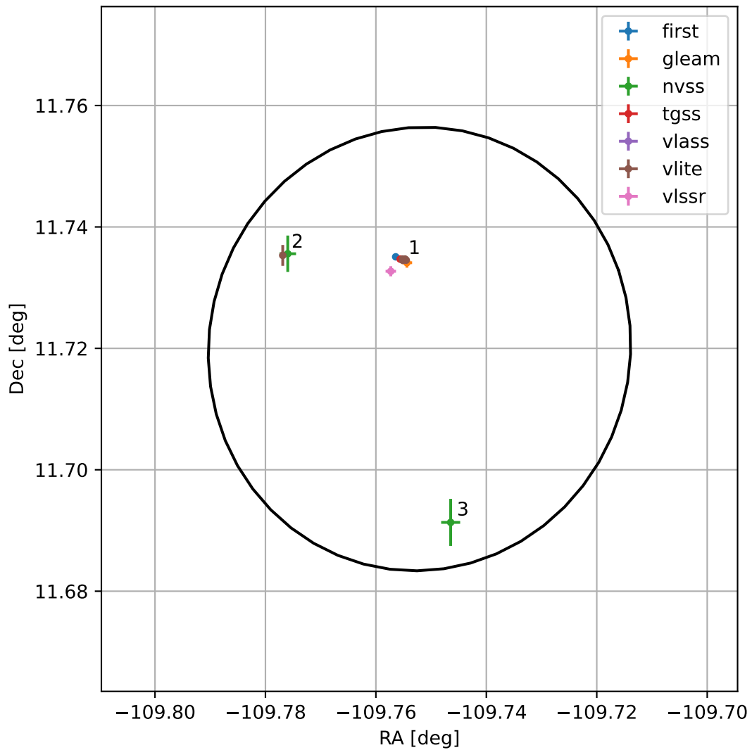
4FGL J1640.9+1143
