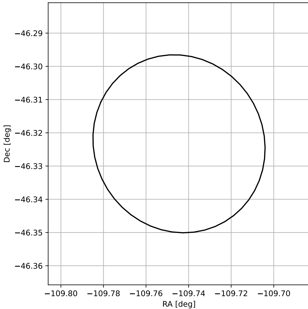
4FGL J1641.0-4619
