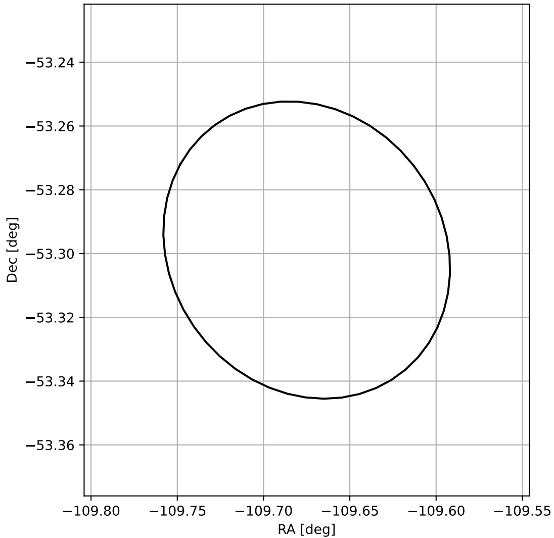
4FGL J1641.2-5317
