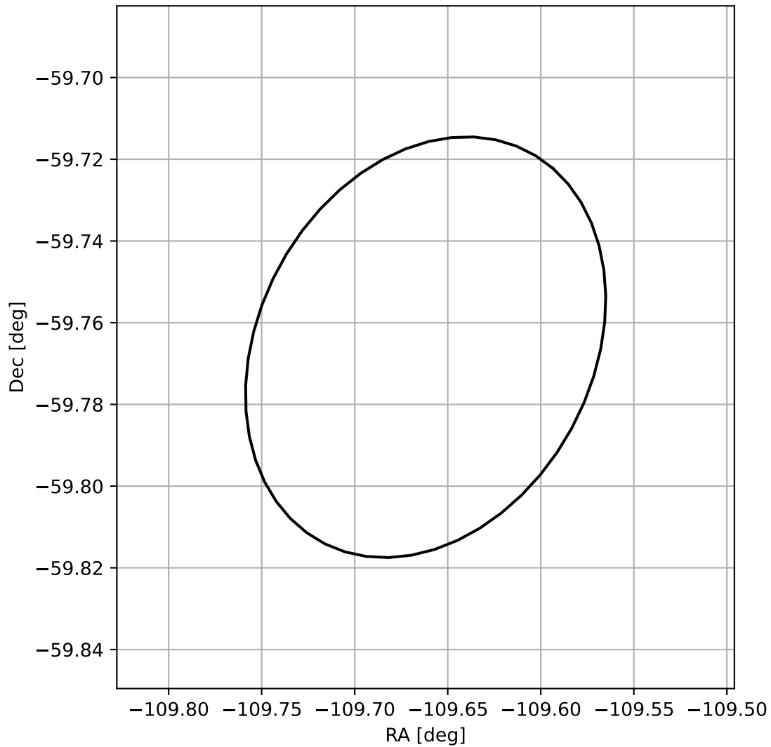
4FGL J1641.3-5945
