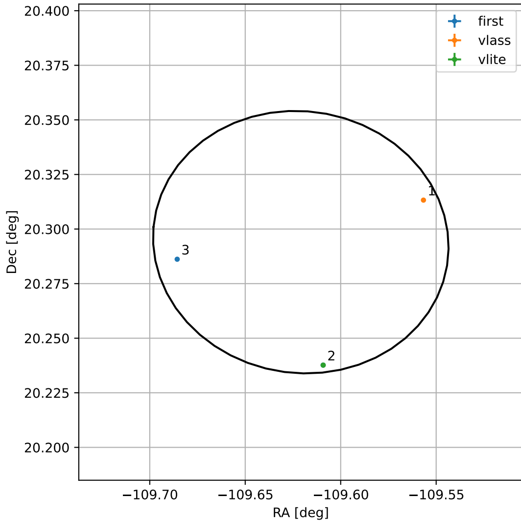
4FGL J1641.5+2017
