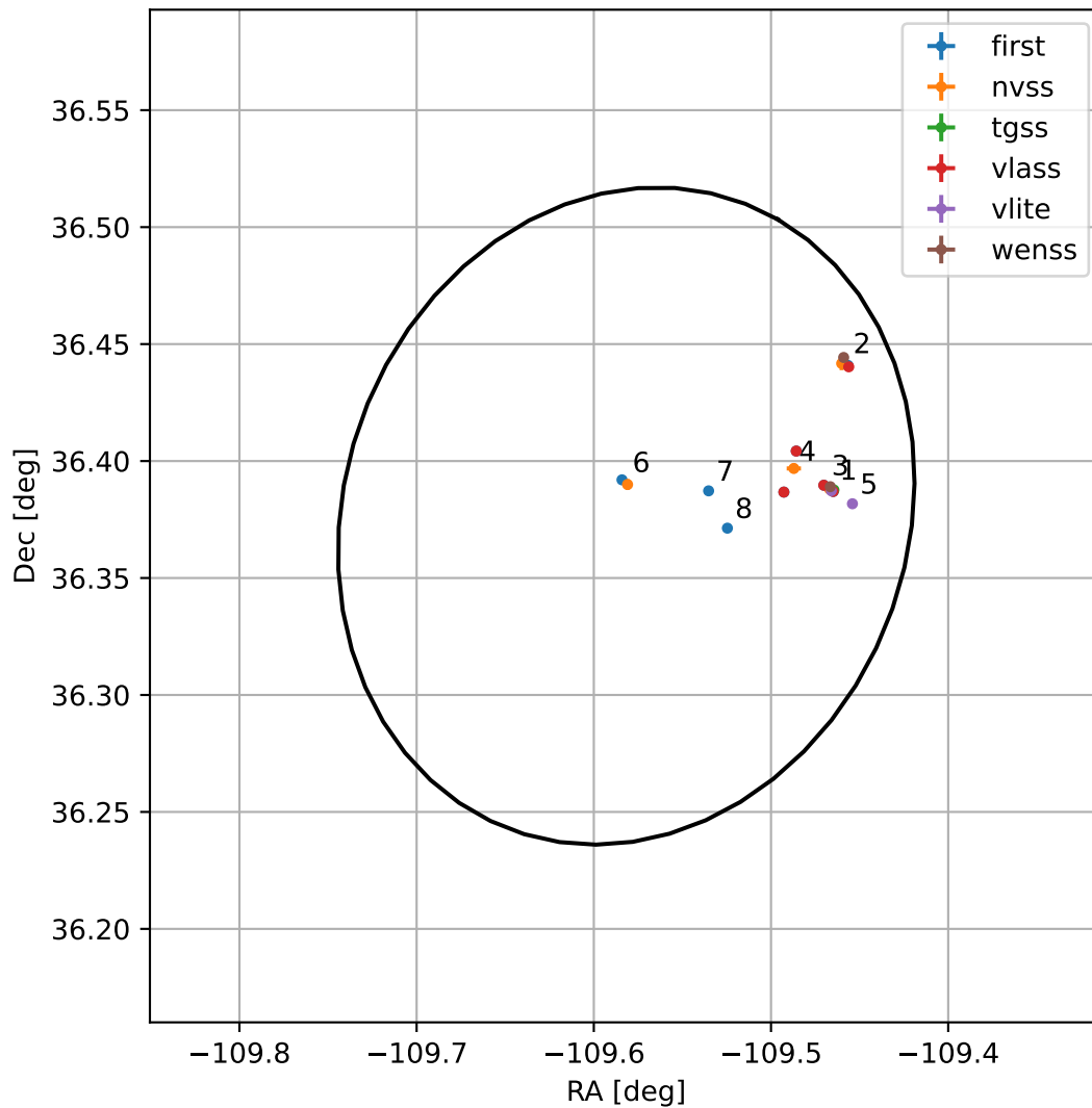
4FGL J1641.6+3622
