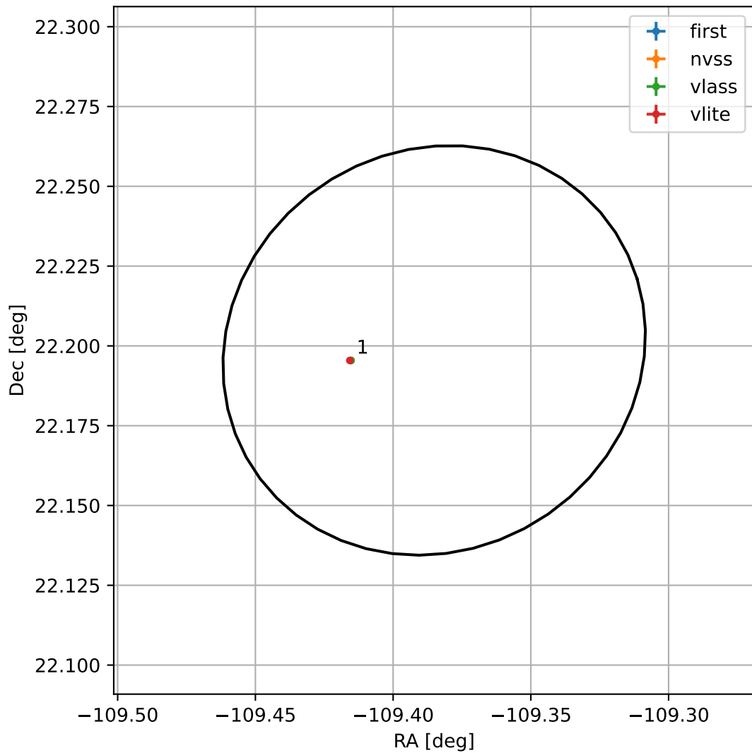
4FGL J1642.4+2211
