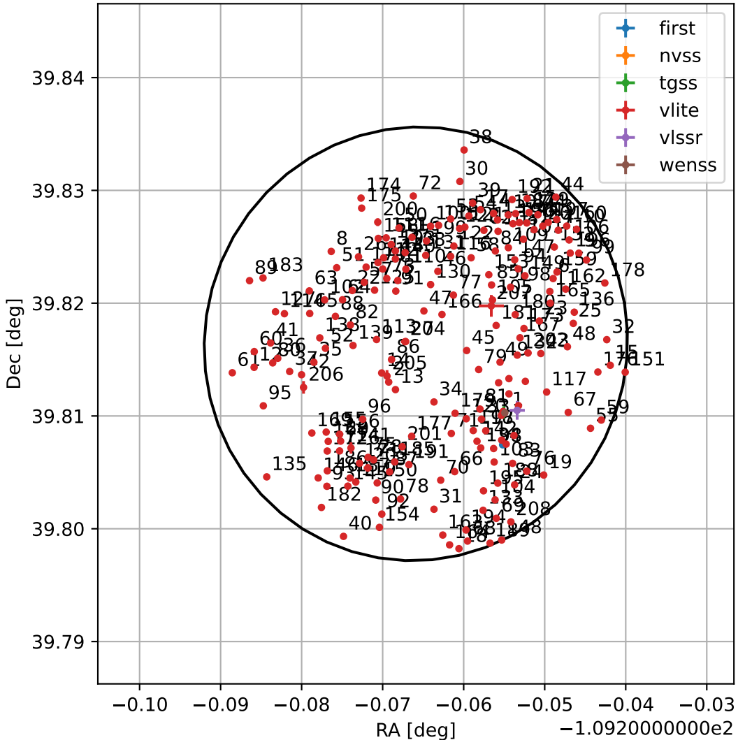
4FGL J1642.9+3948
