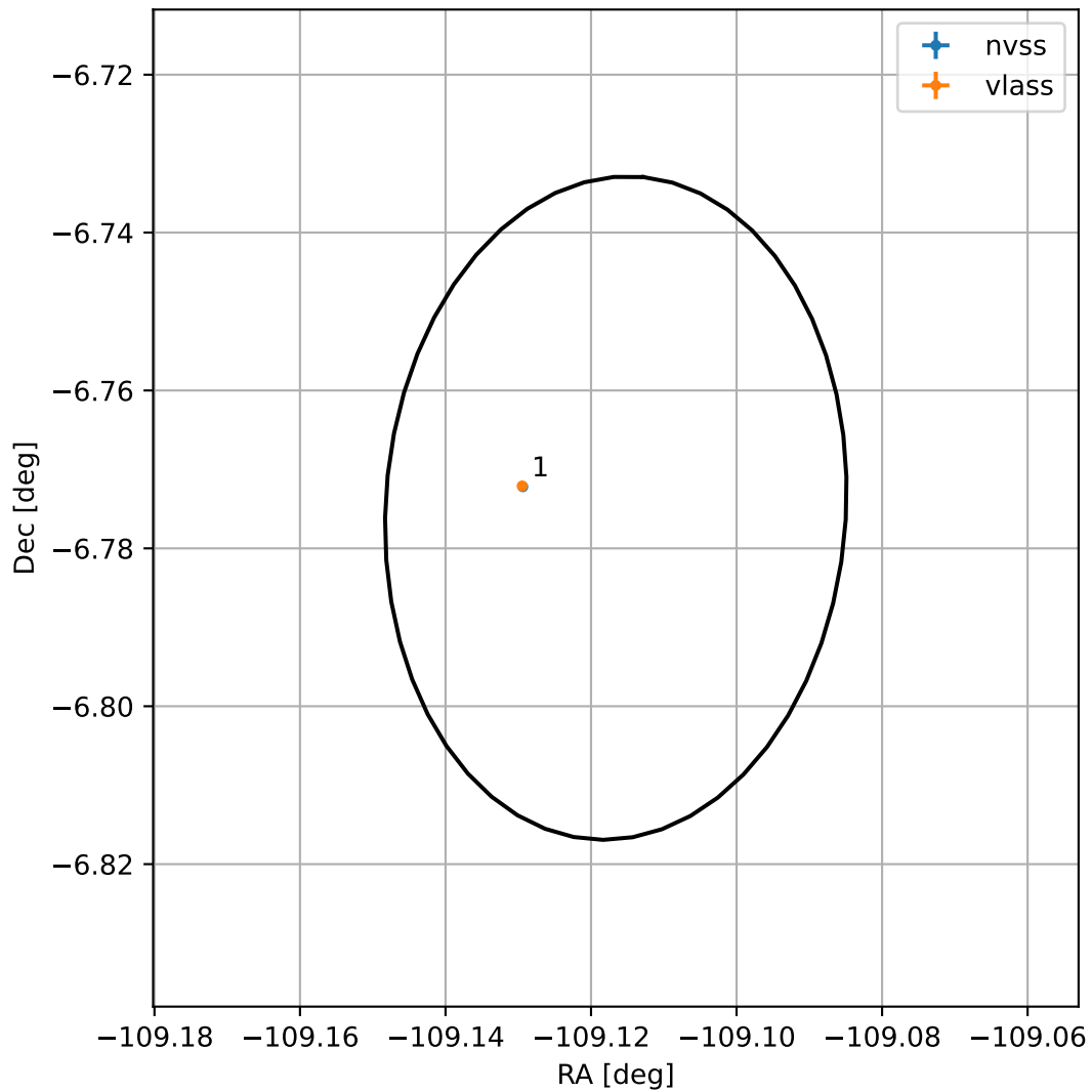
4FGL J1643.5-0646
