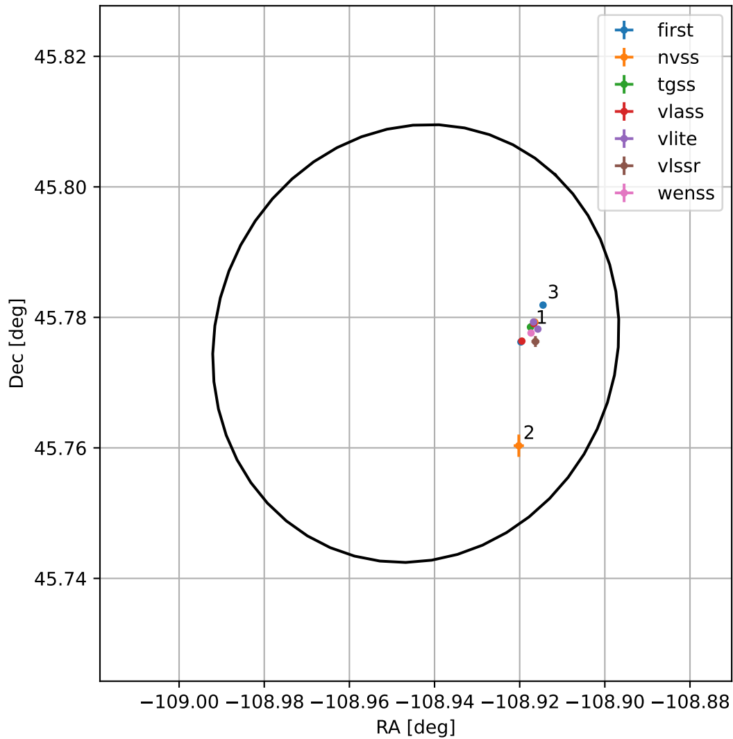
4FGL J1644.2+4546
