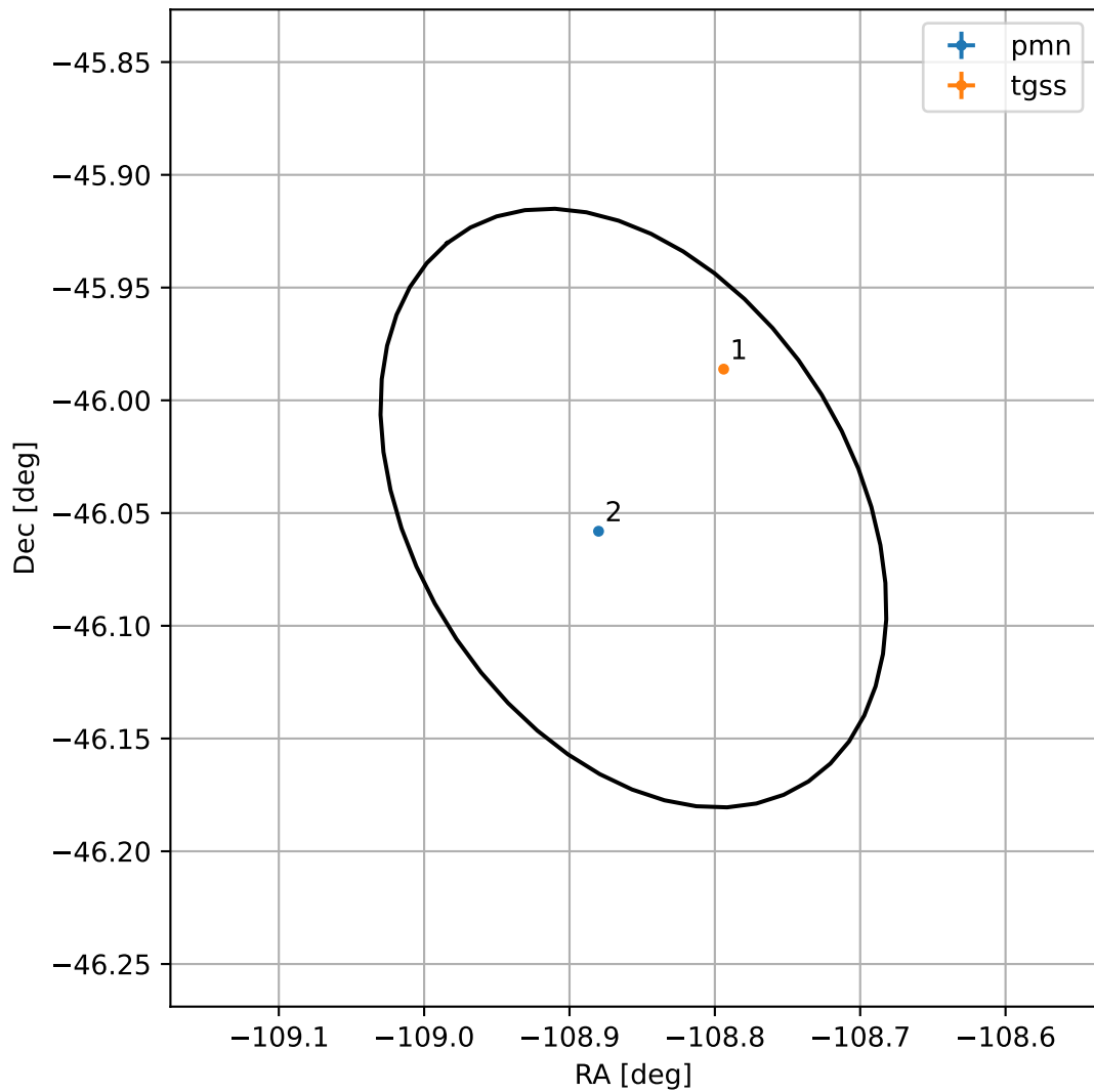
4FGL J1644.5-4602
