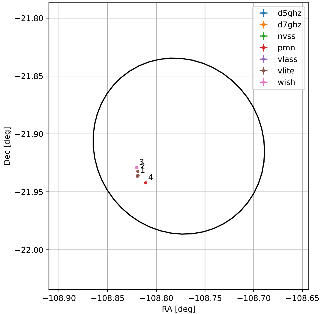
4FGL J1644.8-2154
