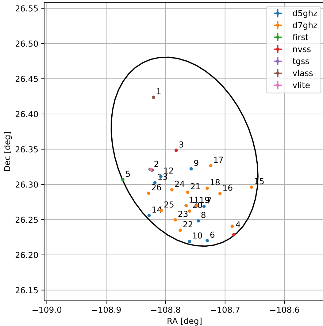
4FGL J1644.9+2620
