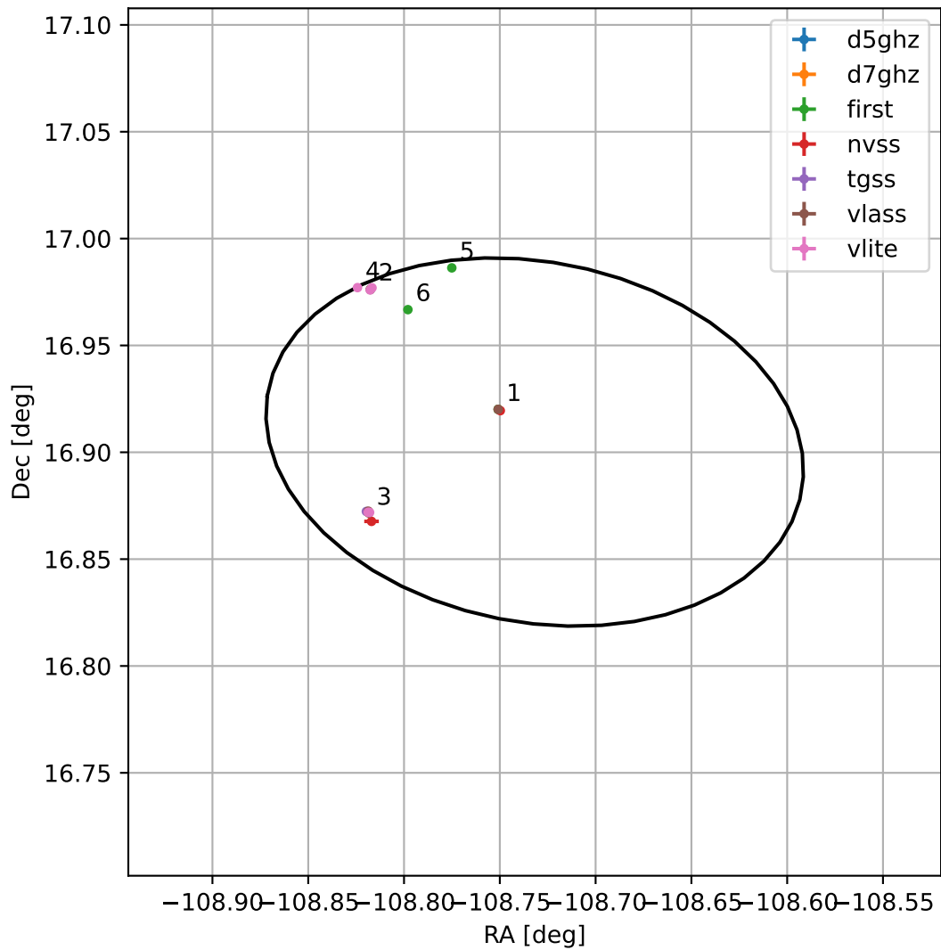
4FGL J1645.0+1654
