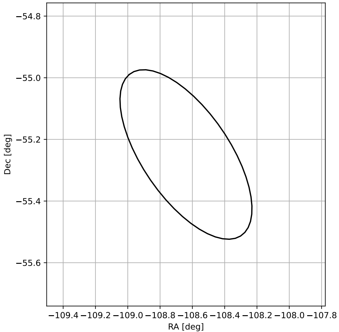
4FGL J1645.4-5514
