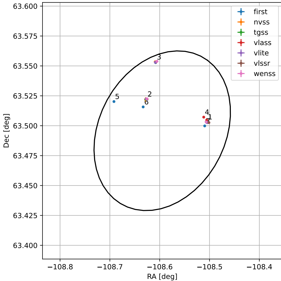
4FGL J1645.6+6329
