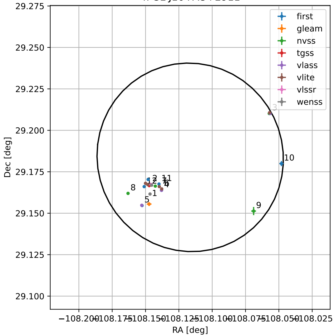
4FGL J1647.5+2911
