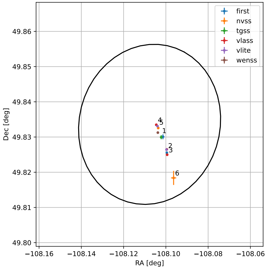
4FGL J1647.5+4950
