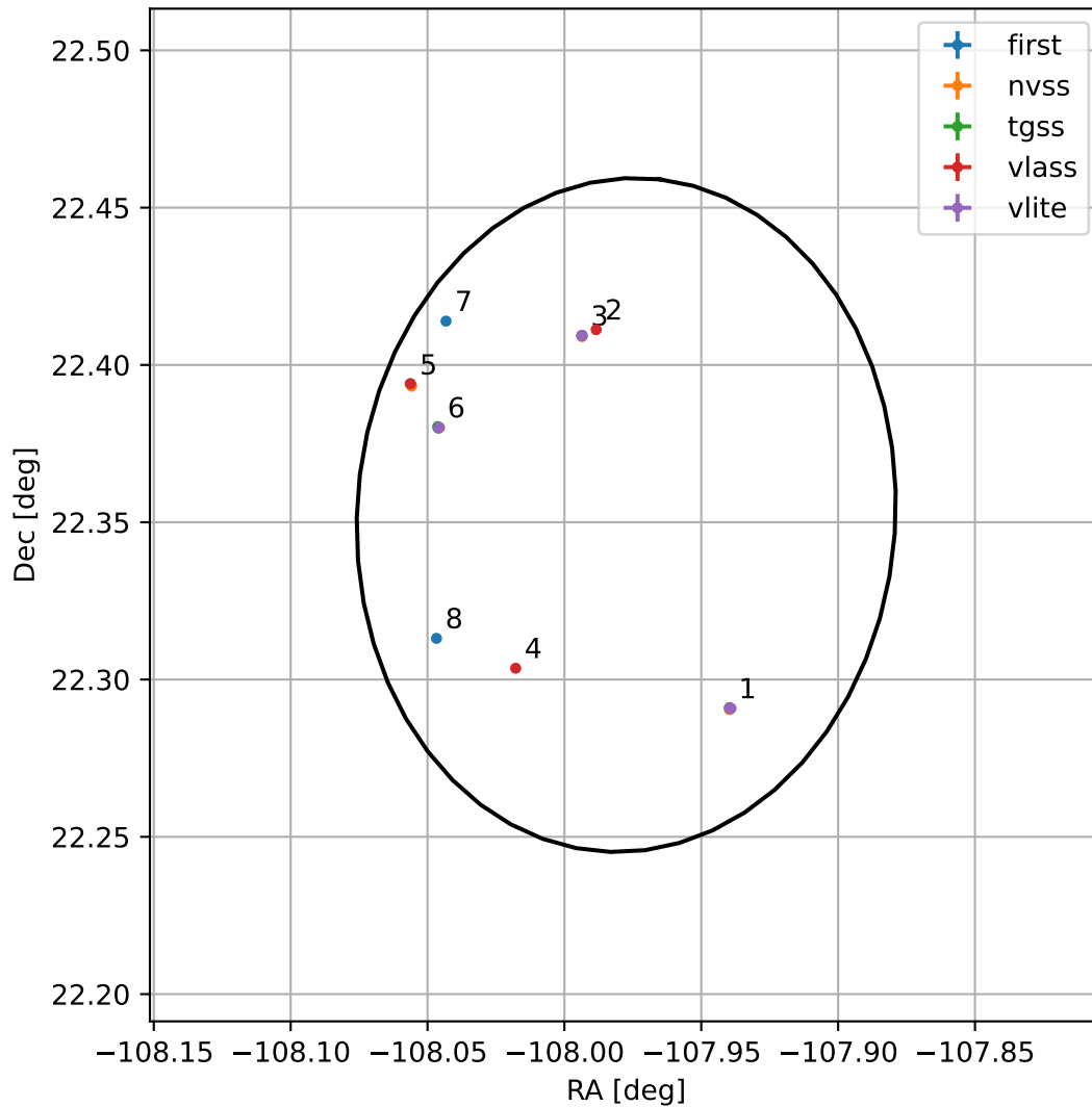
4FGL J1648.0+2221
