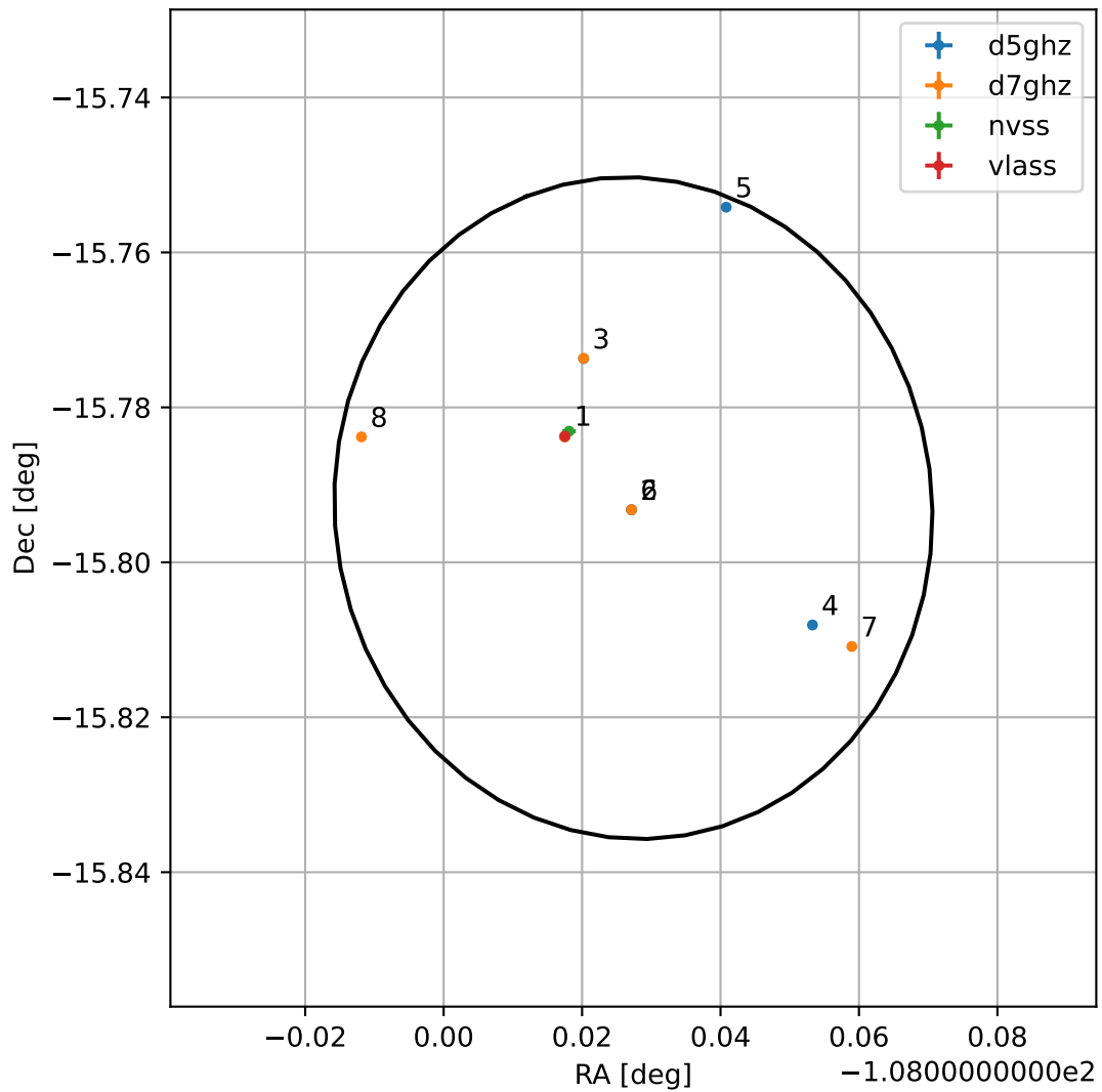
4FGL J1648.1-1547
