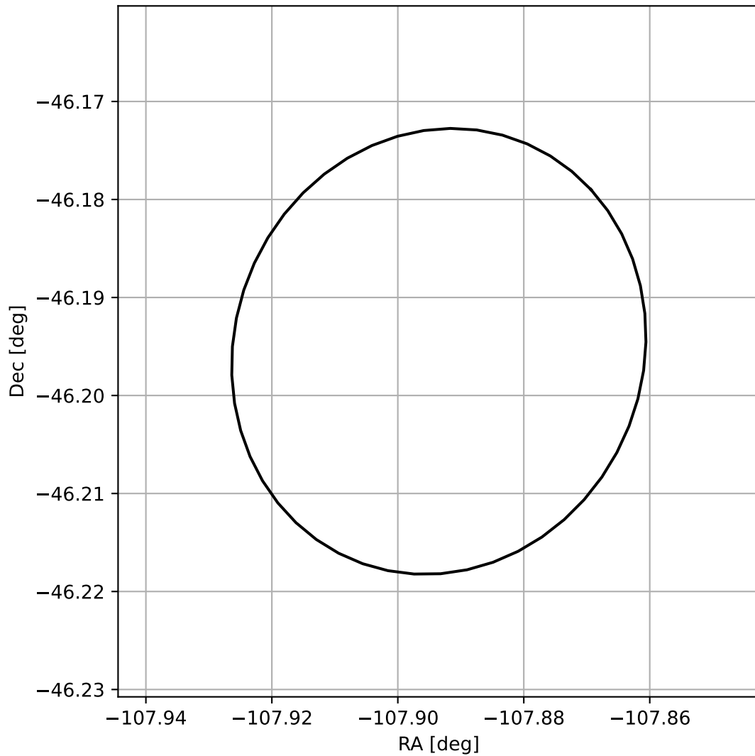
4FGL J1648.4-4611
