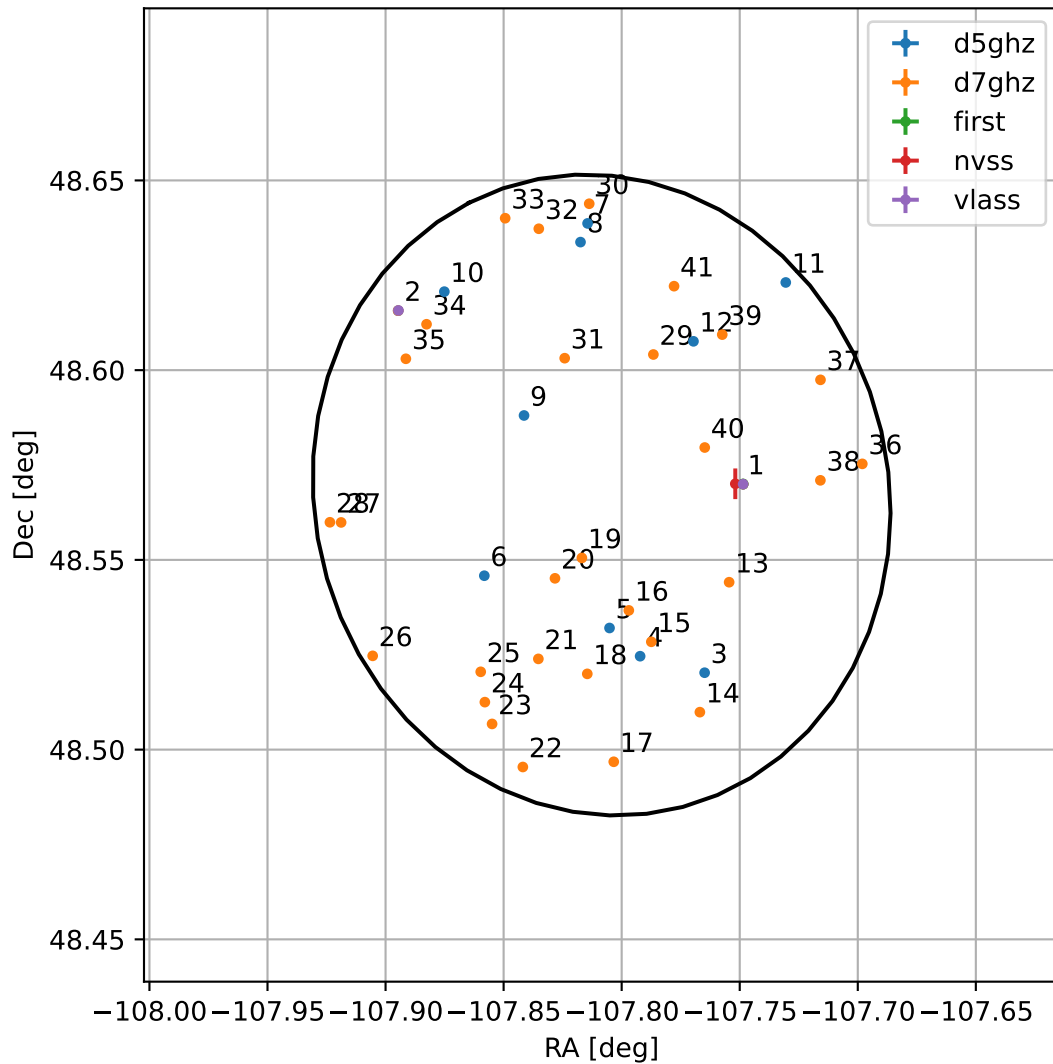
4FGL J1648.7+4834
