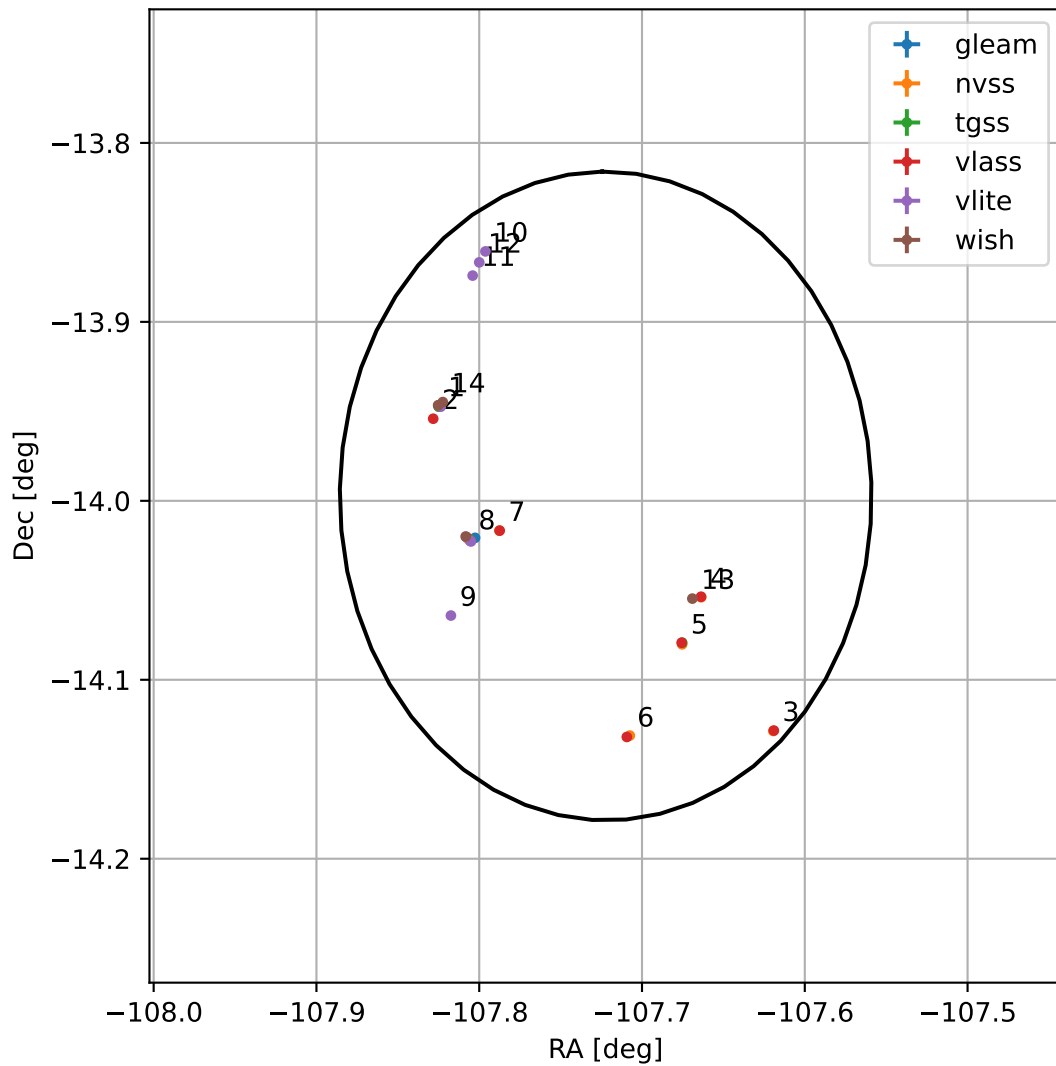
4FGL J1649.1-1359
