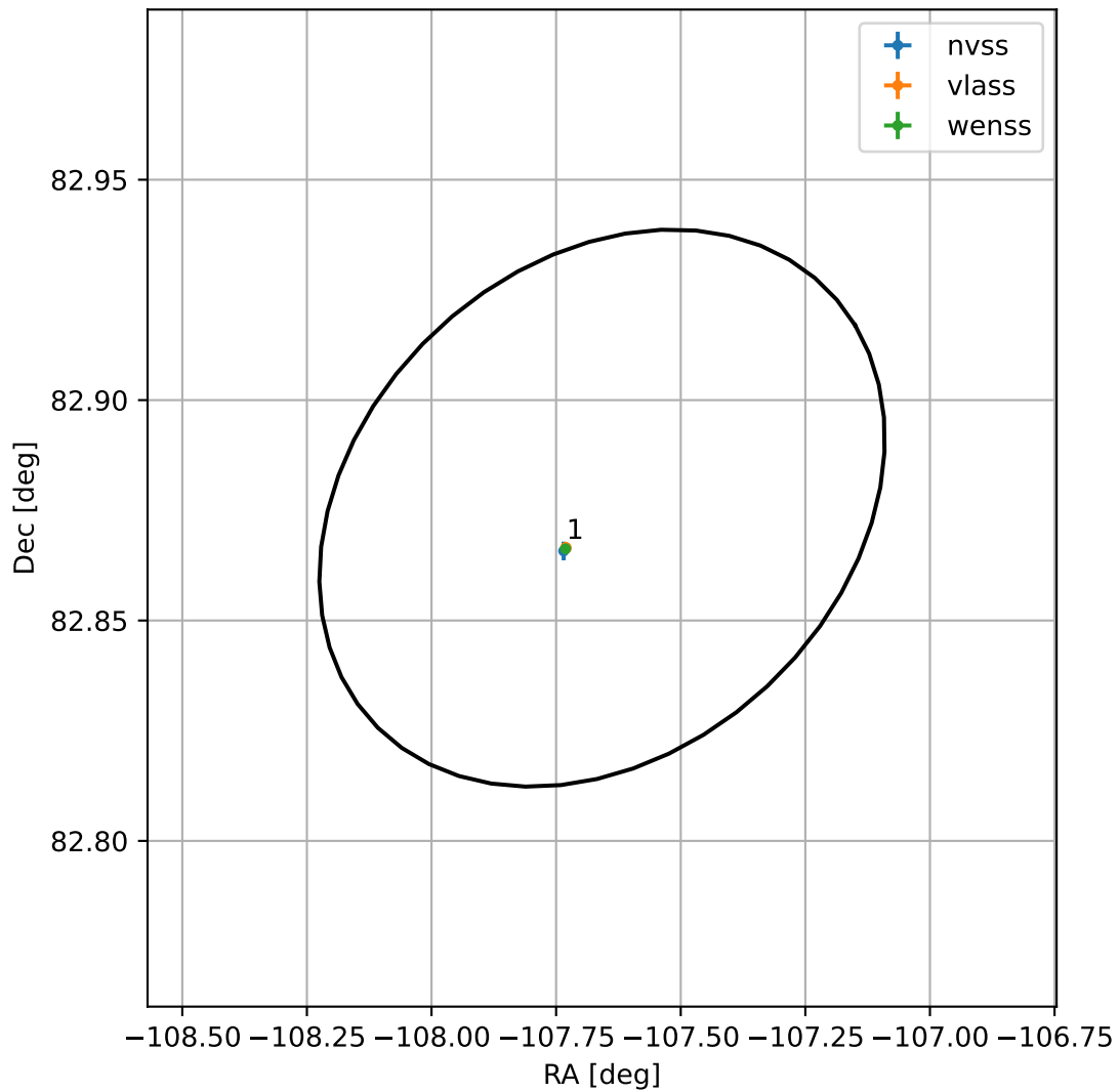
4FGL J1649.3+8252
