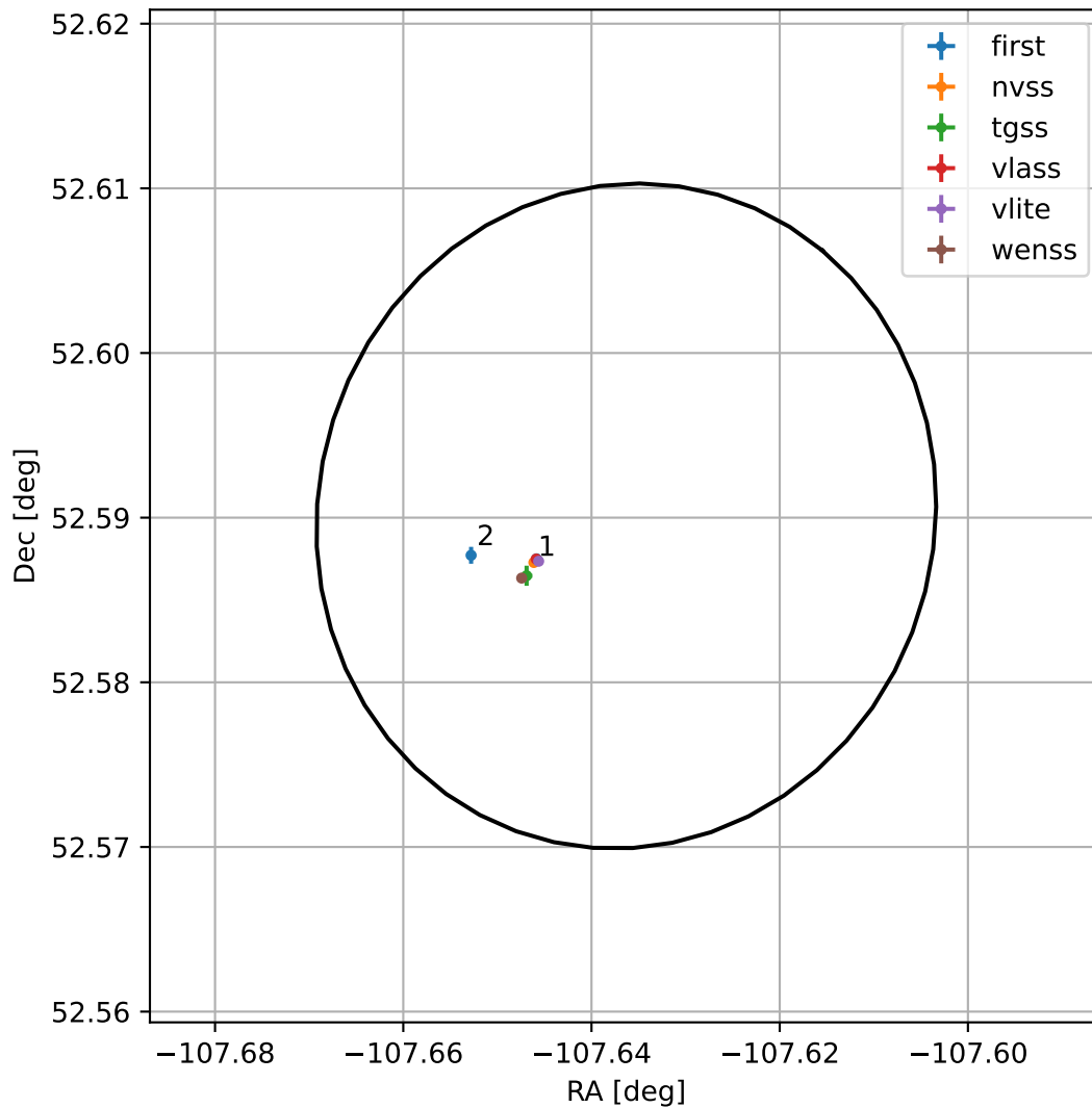
4FGL J1649.4+5235
