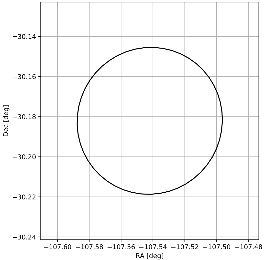
4FGL J1649.8-3010
