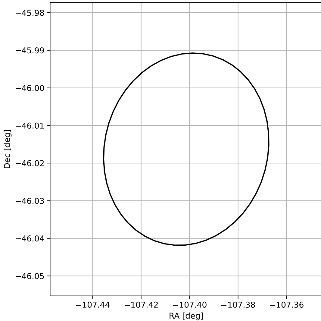
4FGL J1650.3-4600
