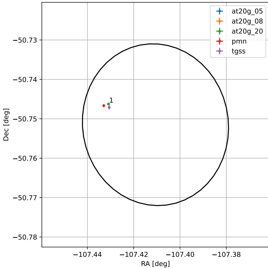
4FGL J1650.3-5045
