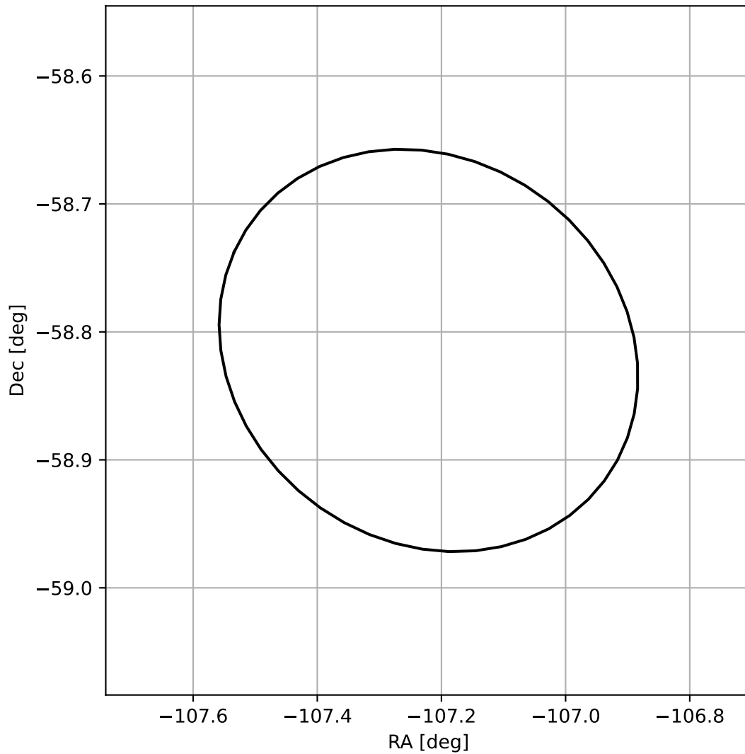
4FGL J1651.1-5848
