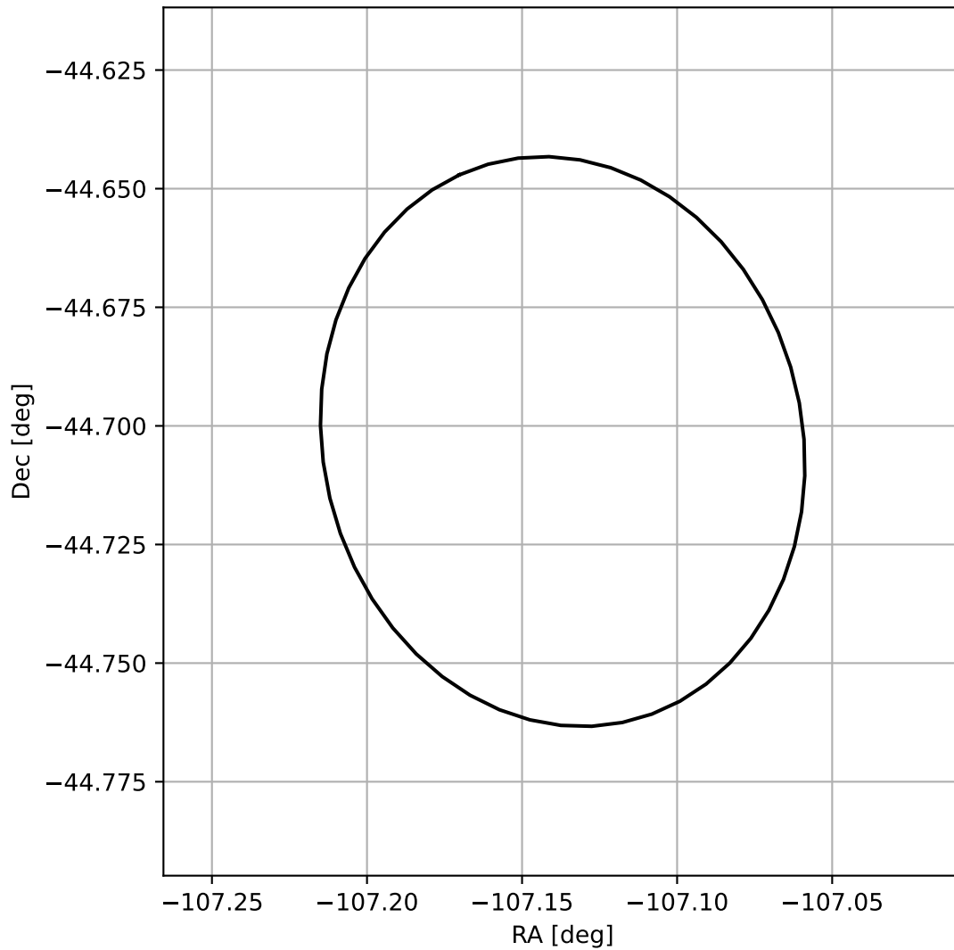
4FGL J1651.4-4442
