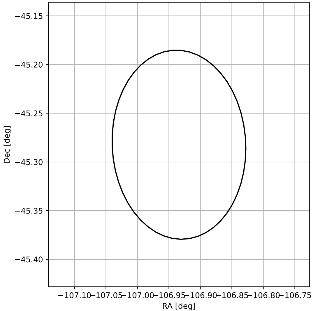
4FGL J1652.2-4516
